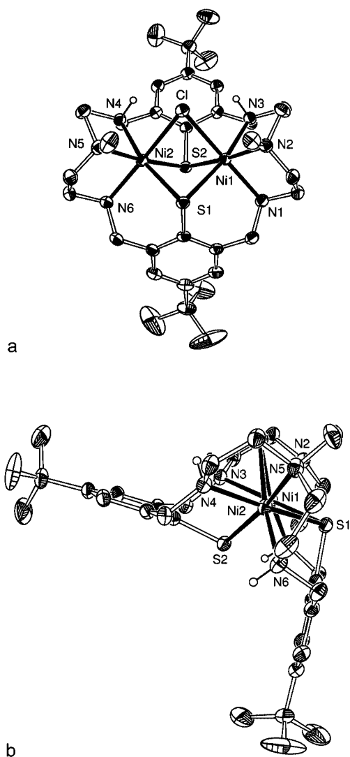
Figure 2. Two perspective views of the molecular structure of 8 with atomic numbering for key atoms (30% probability thermal ellipsoids). Hydrogen atoms (except those bonded to N atoms) have been omitted for clarity.
