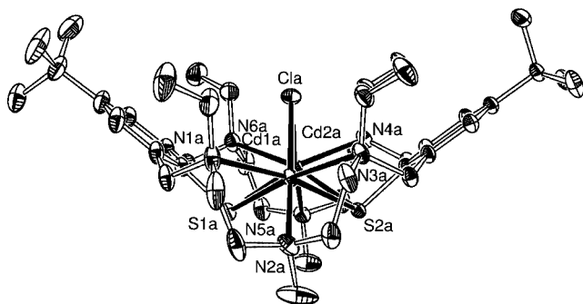
Figure 6. Molecular structure of 13 with atomic numbering for key atoms (30% probability thermal ellipsoids). Hydrogen atoms have been omitted for clarity.
