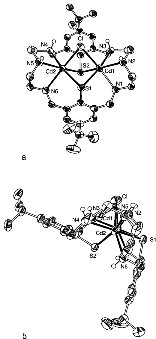
Figure 4. Two perspective views of the molecular structure of 10 with atomic numbering for key atoms (30% probability thermal ellipsoids). Hydrogen atoms (except those bonded to N atoms) have been omitted for clarity.
