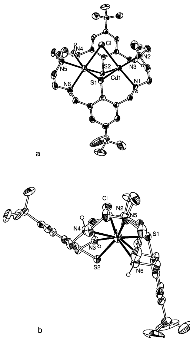
Figure 5. Two perspective views of the molecular structure of 12 with atomic numbering for key atoms (30% probability thermal ellipsoids). Hydrogen atoms (except those bonded to N atoms) have been omitted for clarity.
