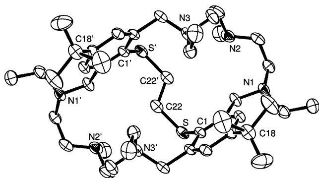
Figure 1. Molecular structure of compound 5 with atomic numbering for key atoms. Hydrogen atoms have been omitted for clarity. Symmetry codes used to generate equivalent atoms: -x, +y, 0.5 - z ( ' ).
