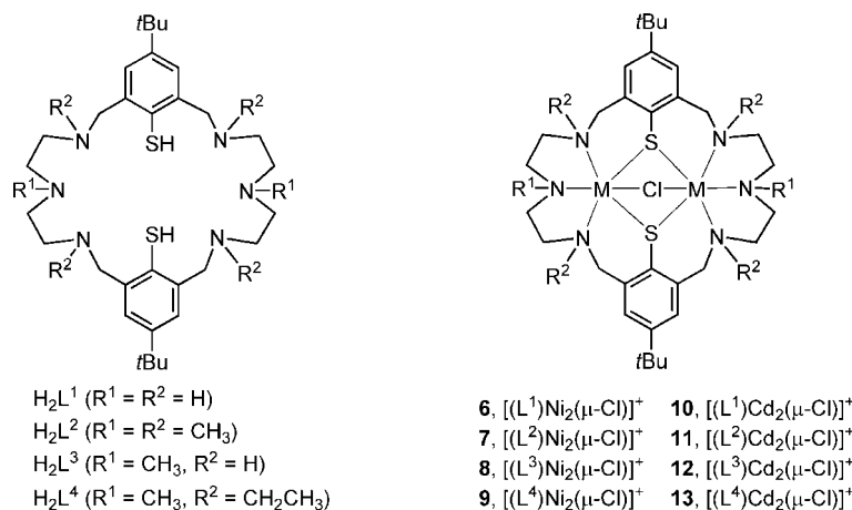
Scheme 1. Ligands and complexes studied in this work.
