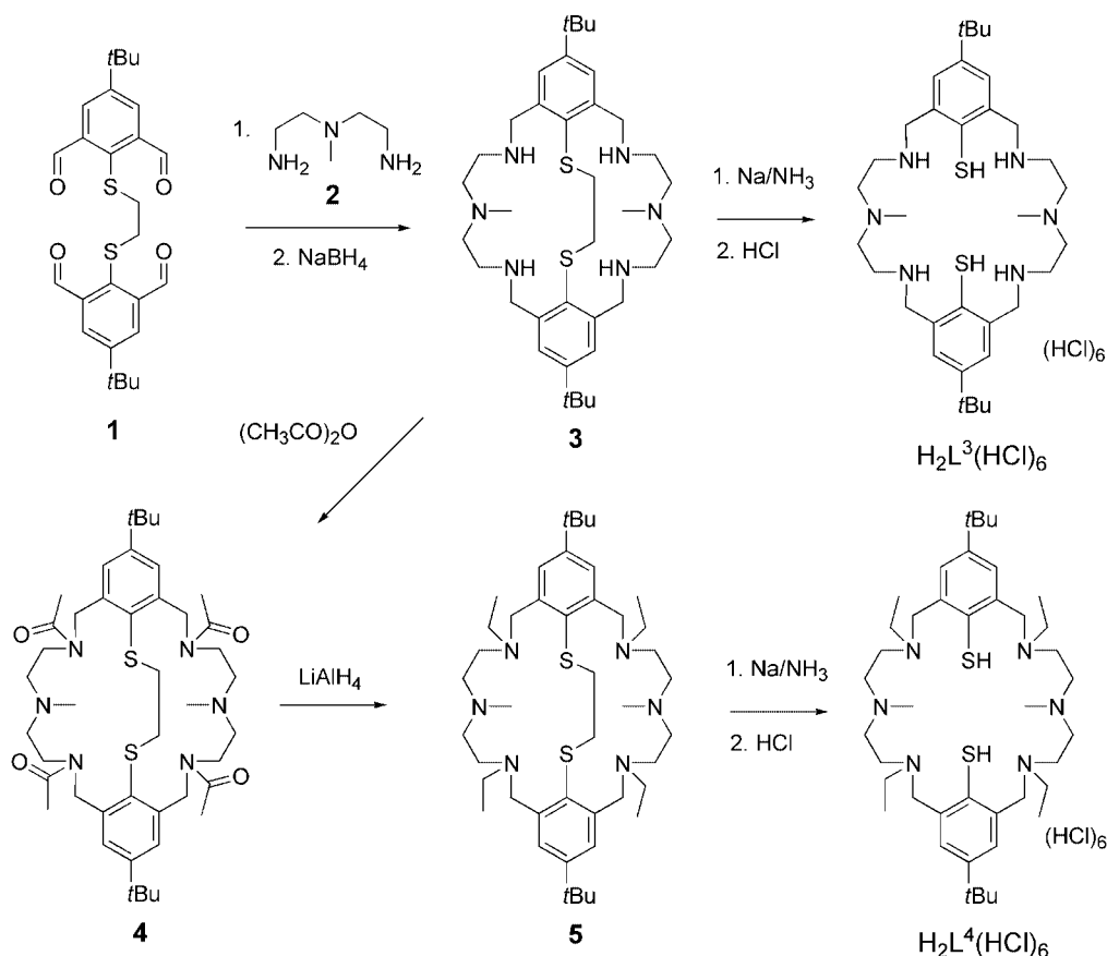
Scheme 3. Synthesis of the ligands H_2L^3 and H_2L^4 .
