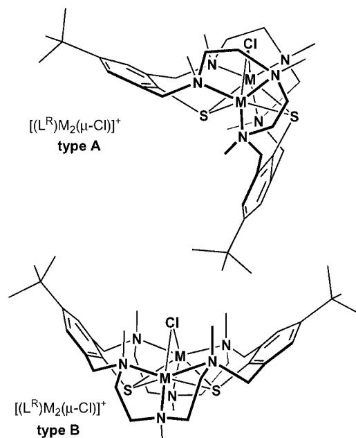
Scheme 2. Schematic representation of the two ligand conformations of the octadentate macrocycles (L^R)^{2-} observed in the chlorido-bridged [(L^R)M_2(\mu-Cl)]^+ complexes 6 , 7 and 11 . [11,13]
