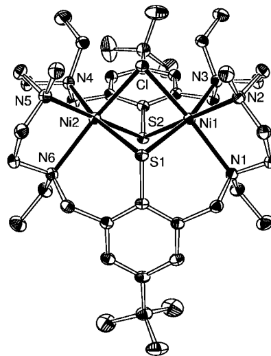
Figure 3. Molecular structure of 9 with atomic numbering for key atoms (30% probability thermal ellipsoids). Hydrogen atoms have been omitted for clarity.
